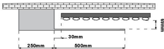
630 X 1800 PALESA UNIVERSAL HANGER MODEL 1 L
