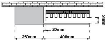
380 X 1800 DIVA UNIVERSAL HANGER MODEL 2 L
