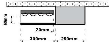
280 X 1800 PALESA UNIVERSAL HANGER MODEL 3 R
