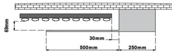
630 X 1800 PALESA UNIVERSAL HANGER MODEL 1 R
