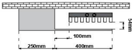
300 X 1800 DIVA UNIVERSAL HANGER MODEL 2 L
