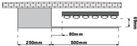
420 X 1800 PALESA UNIVERSAL HANGER MODEL 1 L
