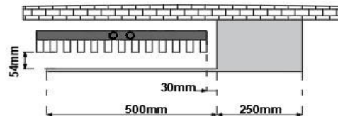
500 X 1800 DIVA UNIVERSAL HANGER MODEL 1 R
