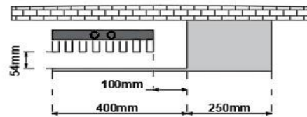
300 X 1800 DIVA UNIVERSAL HANGER MODEL 2 R
