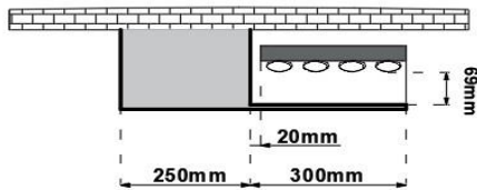
280 X 1800 PALESA UNIVERSAL HANGER MODEL 3 L
