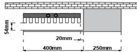
380 X 1800 DIVA UNIVERSAL HANGER MODEL 2 R
